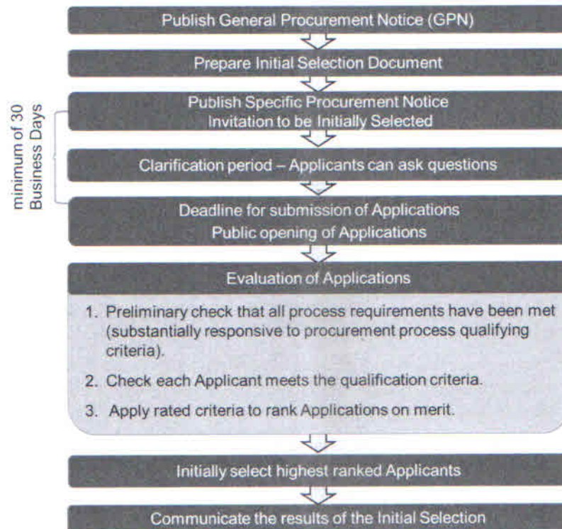
Figure 1: Process flow chart: Initial Selection
